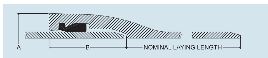
Fastite® Joint
